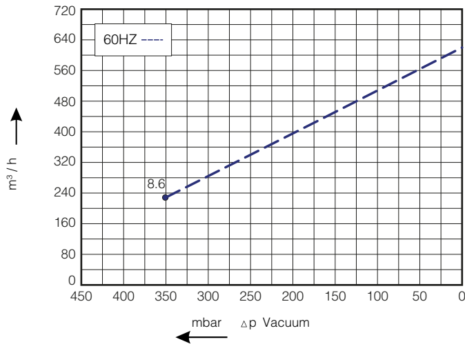
Vacuum Selection Curve
