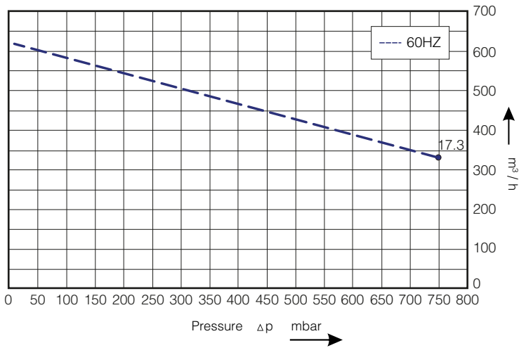
Pressure Selection Curve
