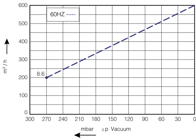
Vacuum Selection Curve
