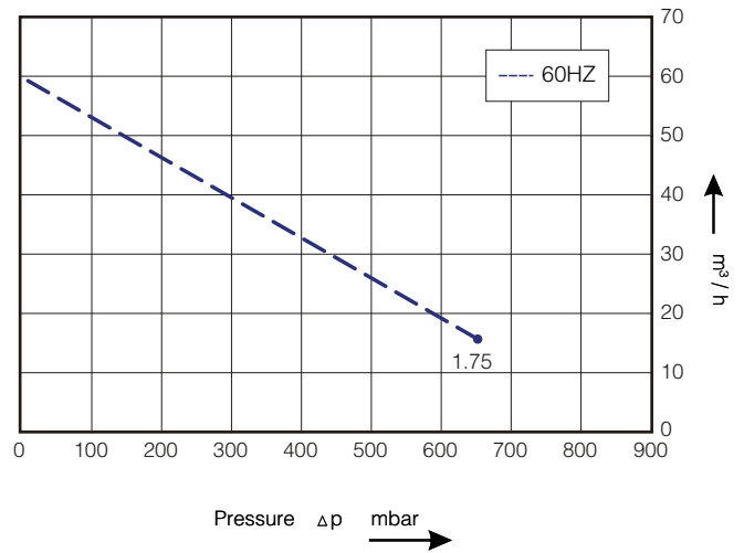
Pressure Selection Curve
