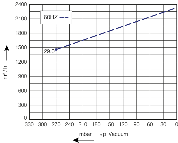
Vacuum Selection Curve
