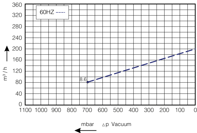
Vacuum Selection Curve
