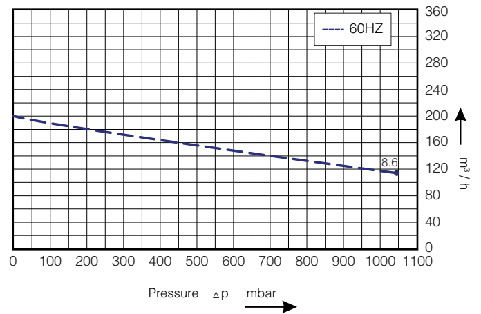
Pressure Selection Curve
